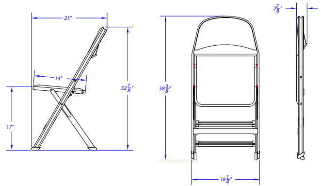
3400C Contour Folding Chair
