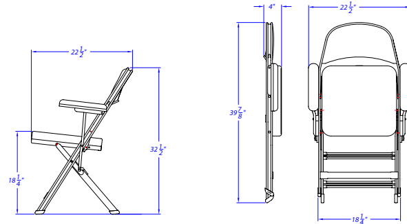
3402B 2-Arm Folding Chair
