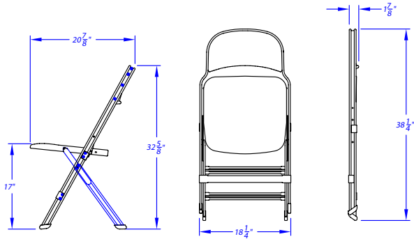
2000S All Steel Folding Chair
