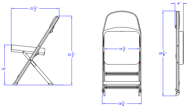
3400FLX Flex Seat Folding Chair
