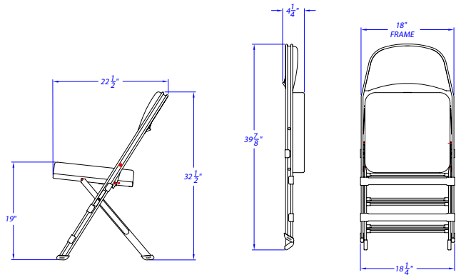
3400B-HD Heavy Duty Folding Chair
